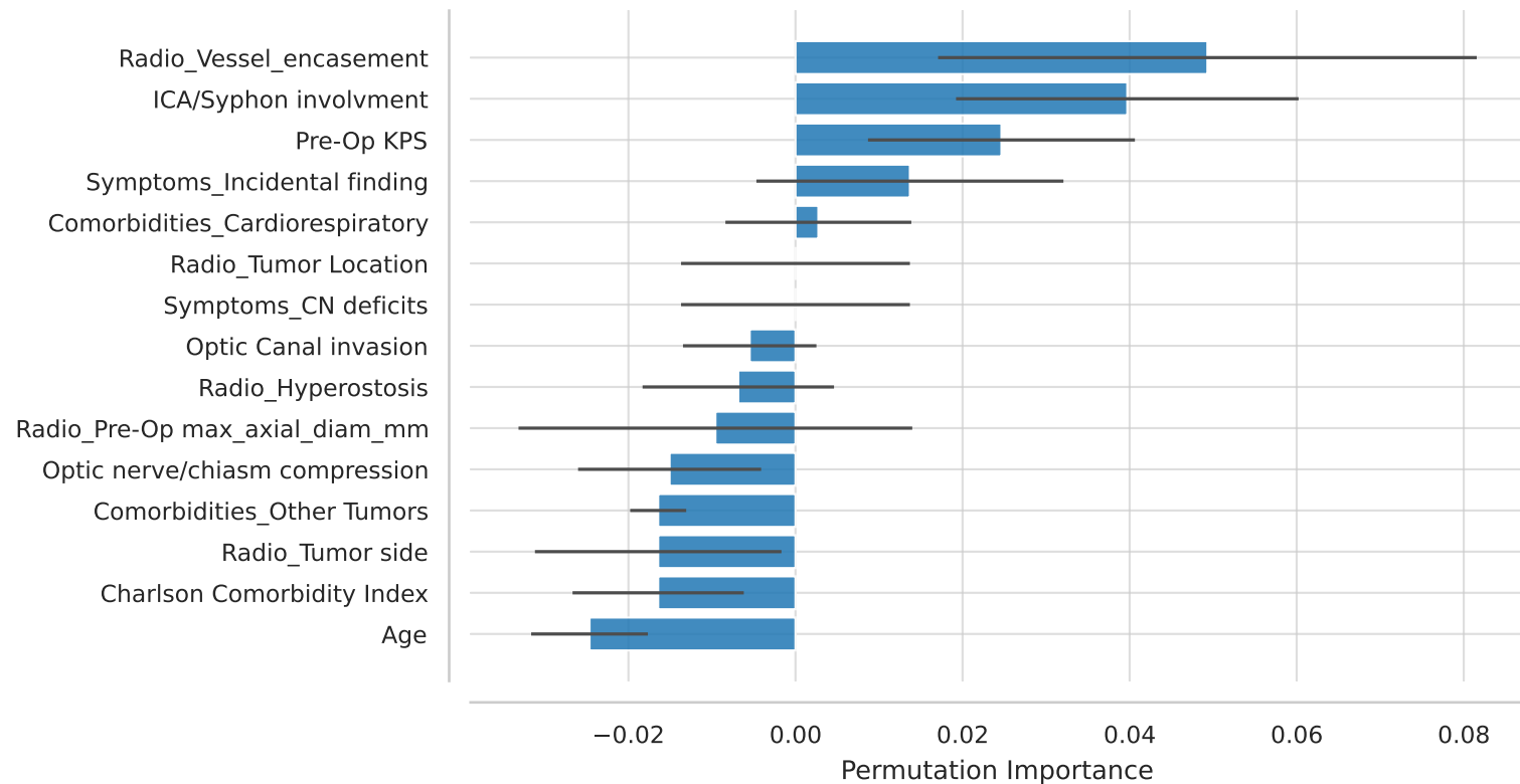
Feature Importance (TORCH_MLP)
